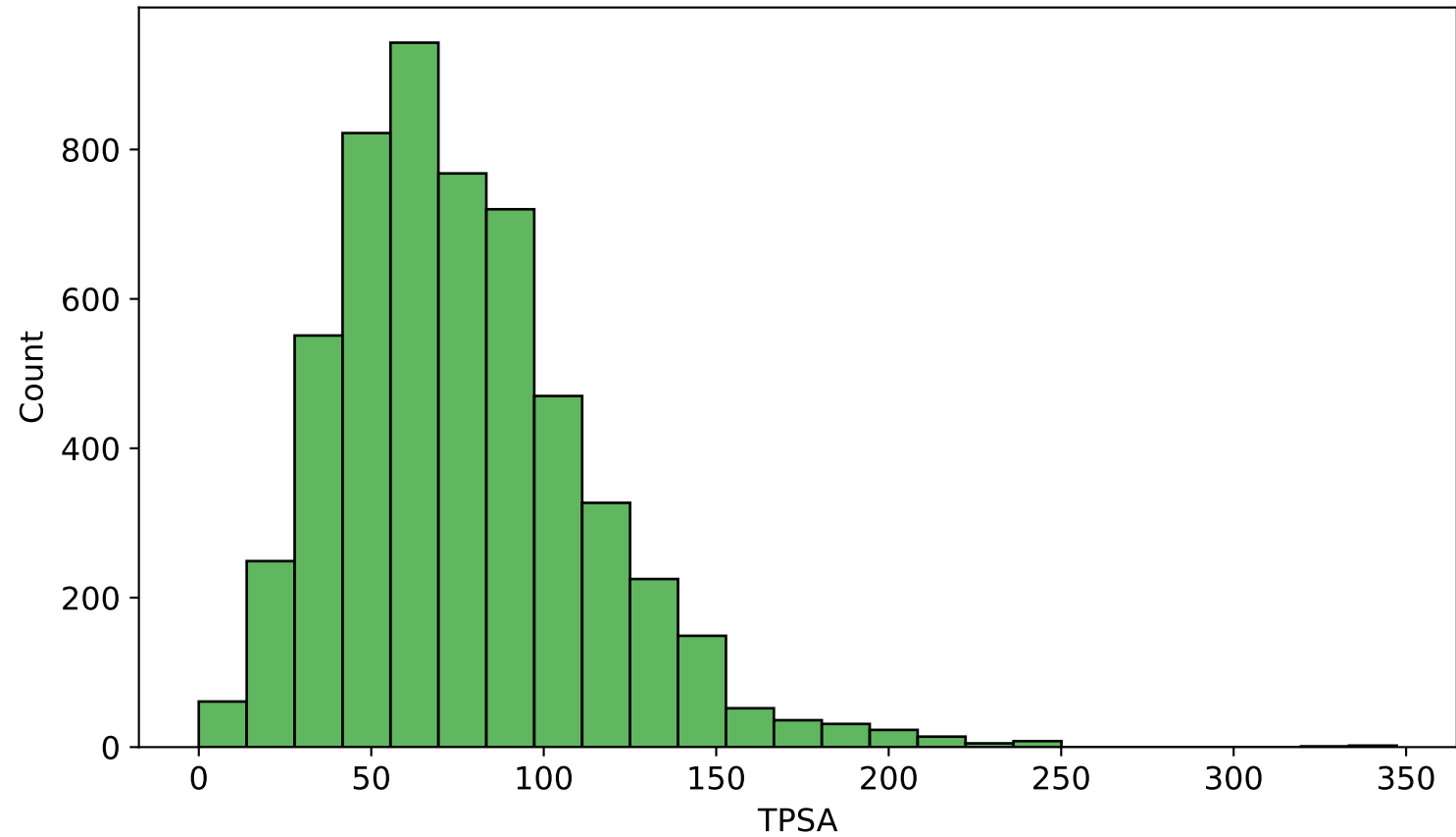
Histogram of TPSA
