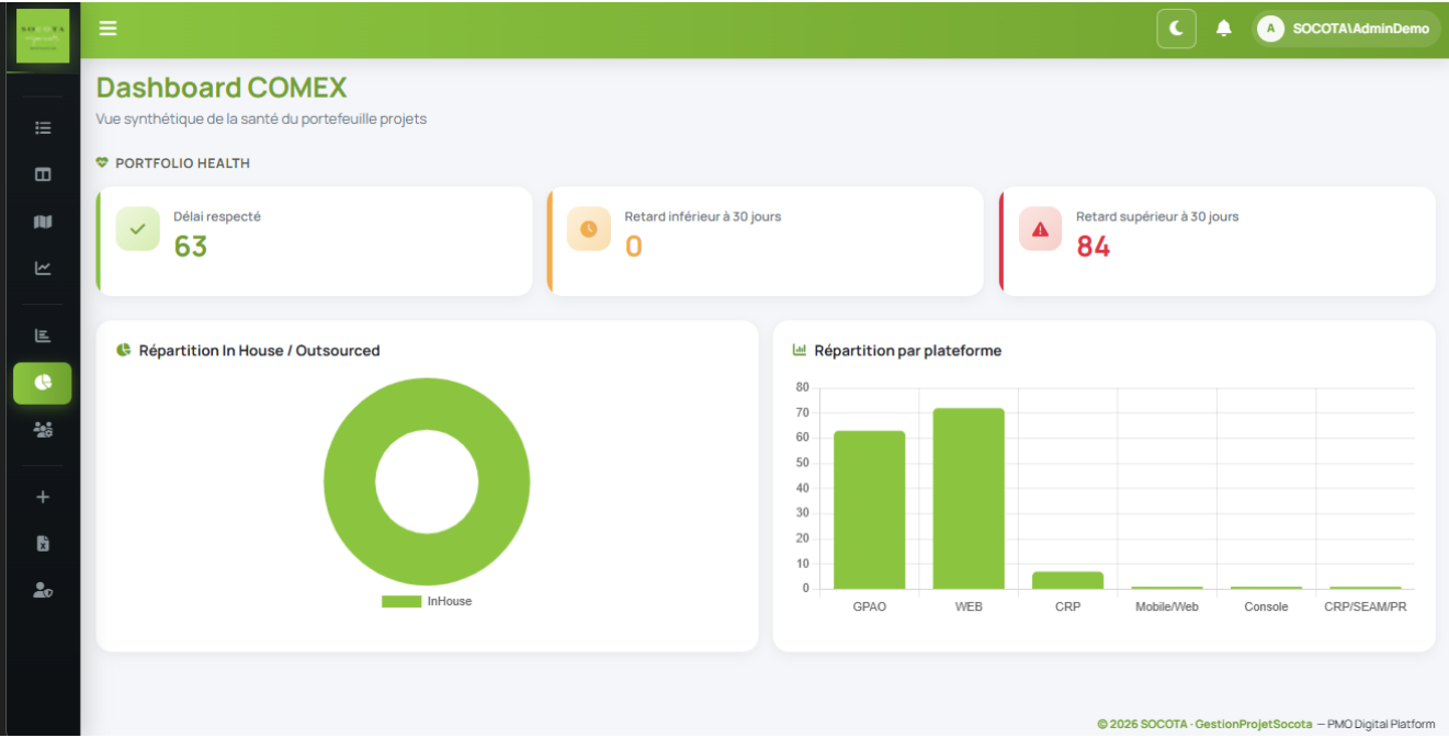
Figure 9 — Dashboard COMEX.
