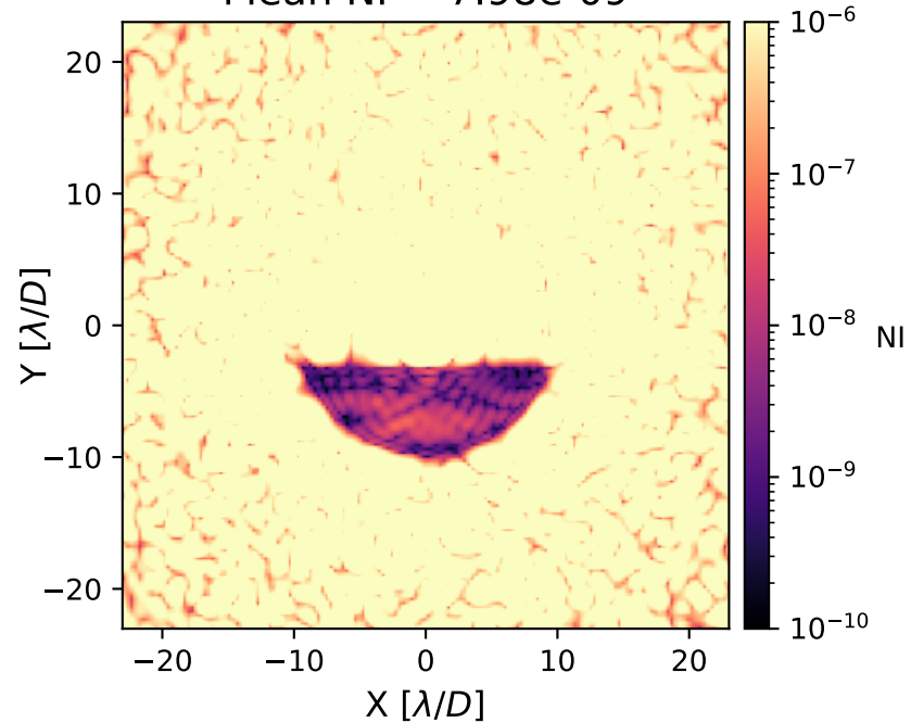
Best Iteration from aEFC SCoOB simulation: Mean NI = 7.98e-09
