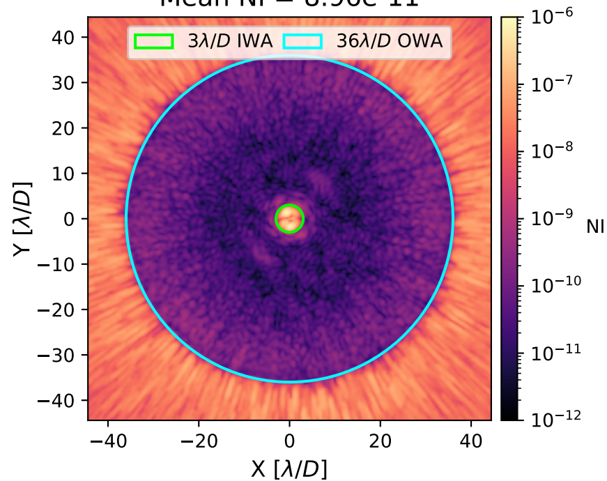
Best aEFC Iteration: Mean NI = 8.96\text{e-}11
