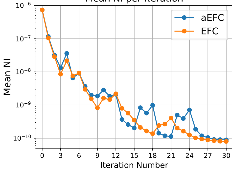
Mean NI per Iteration
