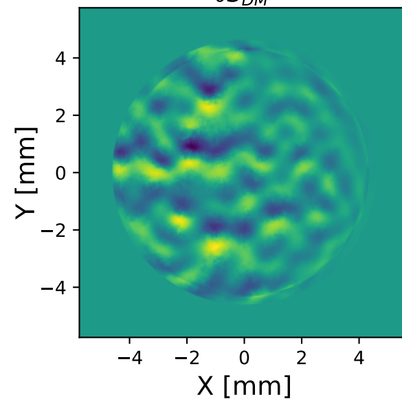
Phase of Gradient at Pre-FPM Pupil
