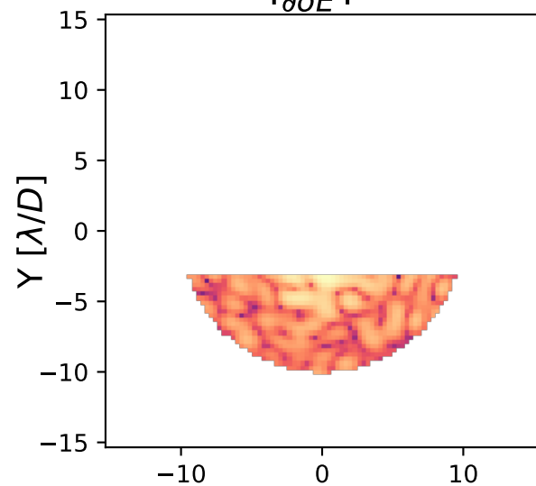
Phase of Gradient at Focal Plane
