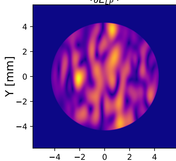
Phase of Gradient at Lyot Pupil
