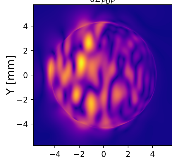
Phase of Gradient at Pre-FPM Pupil
