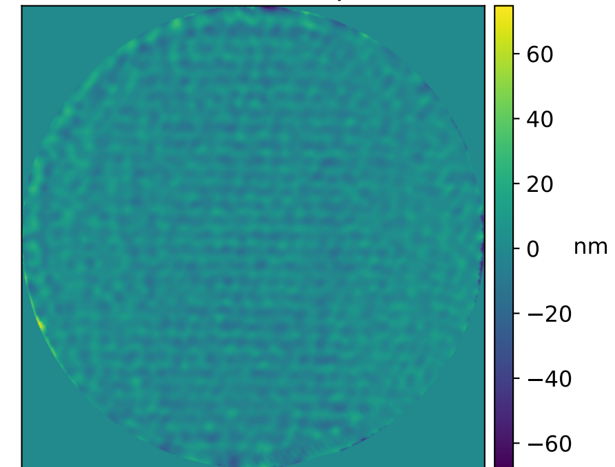
SCoOB Pre-FPM Pupil OPD
