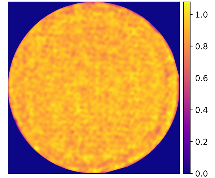
SCoOB Pre-FPM Pupil Amplitude
