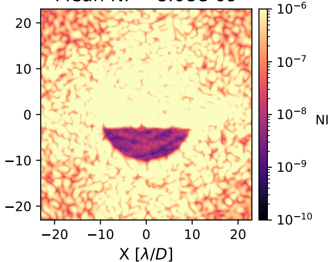
Best Iteration with aEFC: Mean NI = 8.08\text{e-}09
