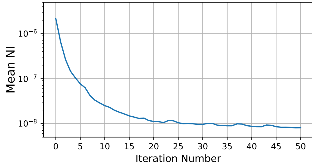
Mean NI per Iteration with aEFC
