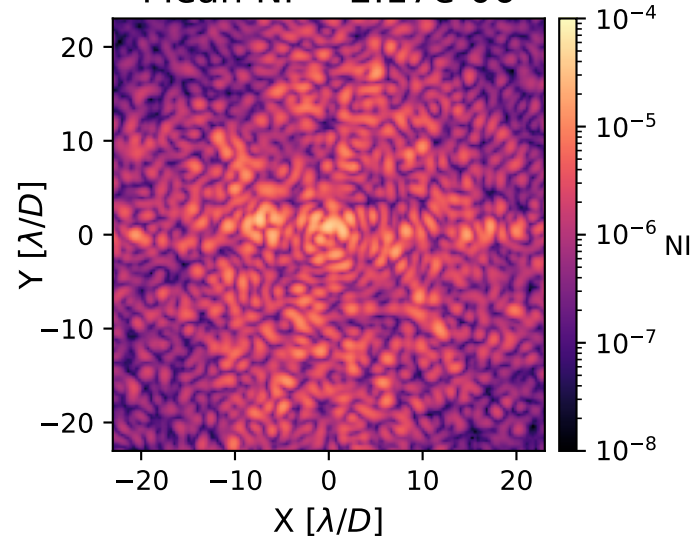
Initial Image: Mean NI = 2.17\text{e-}06
