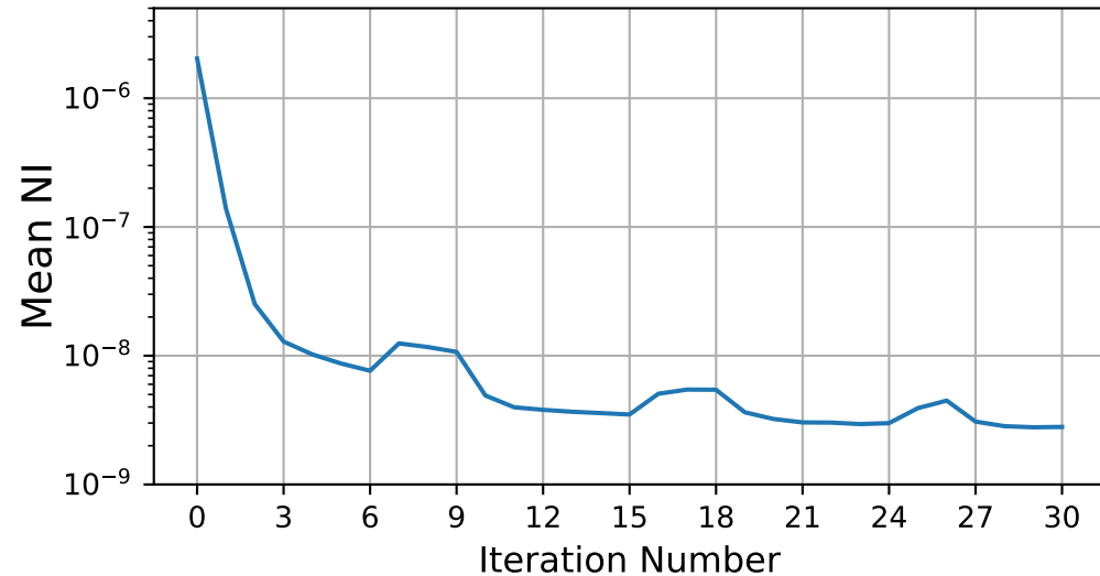
Mean NI per Iteration with iEFC
