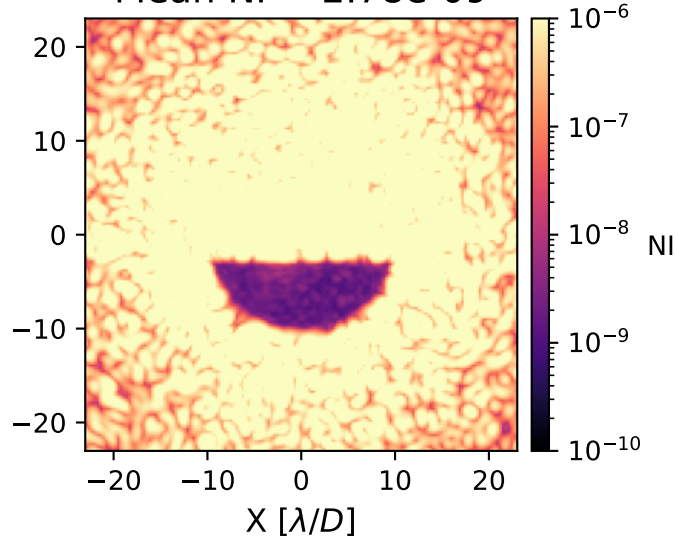
Best Iteration with iEFC: Mean NI = 2.78\text{e-}09
