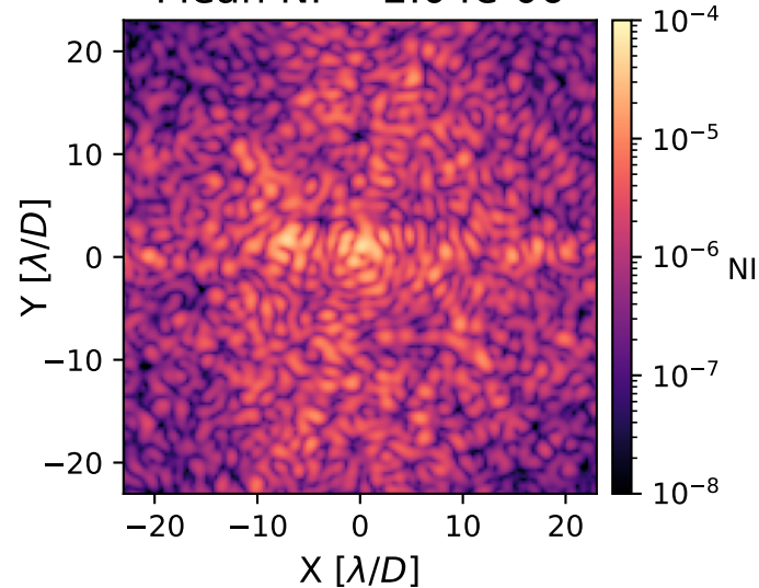
Initial Image: Mean NI = 2.04\text{e-}06
