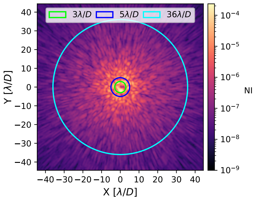
Initial Coronagraphic Image: Total Mean NI = 7.38 \times 10^{-7} 3-5 NI = 1.76 \times 10^{-5}
