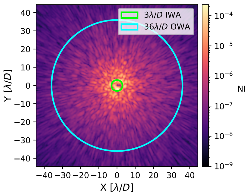
Initial Coronagraphic Image: Mean NI = 7.38 \times 10^{-7}
