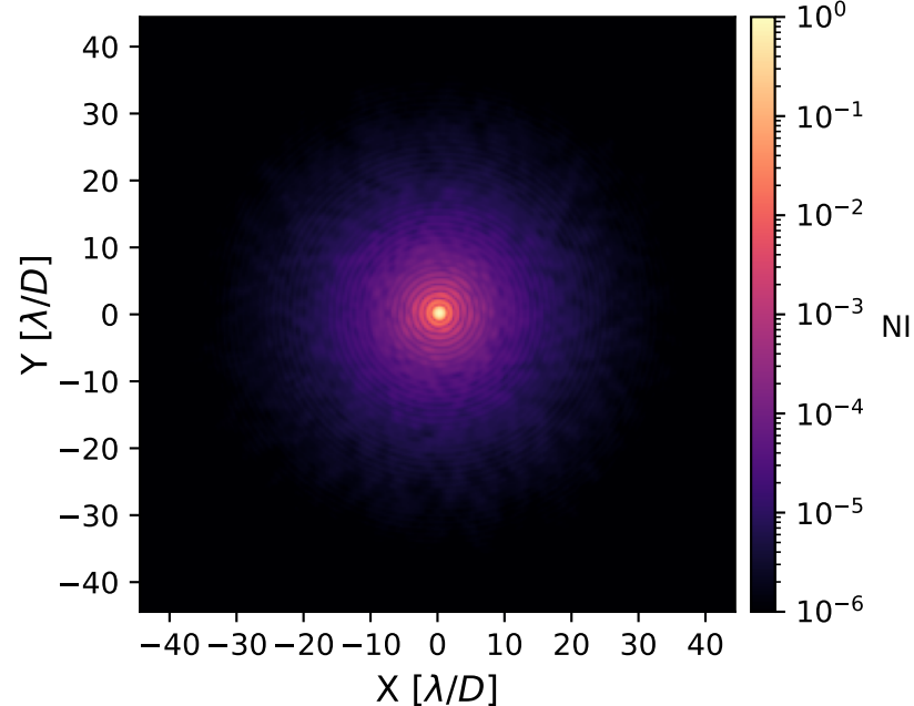
Normalized Reference PSF
