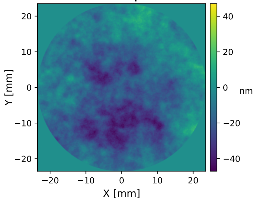
Pre-FPM Pupil OPD
