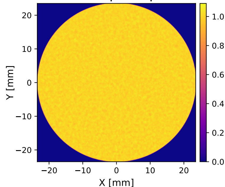
Pre-FPM Pupil Amplitude
