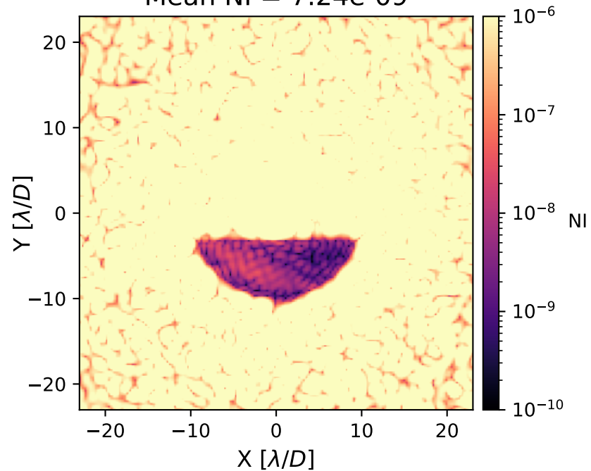
Best Iteration from aEFC SCoOB simulation: Mean NI = 7.24\text{e-}09
