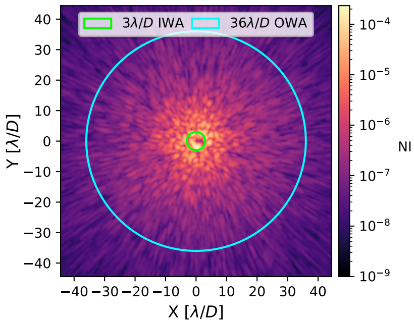
Initial Coronagraphic Image: Total Mean NI = 7.38 \times 10^{-7}
