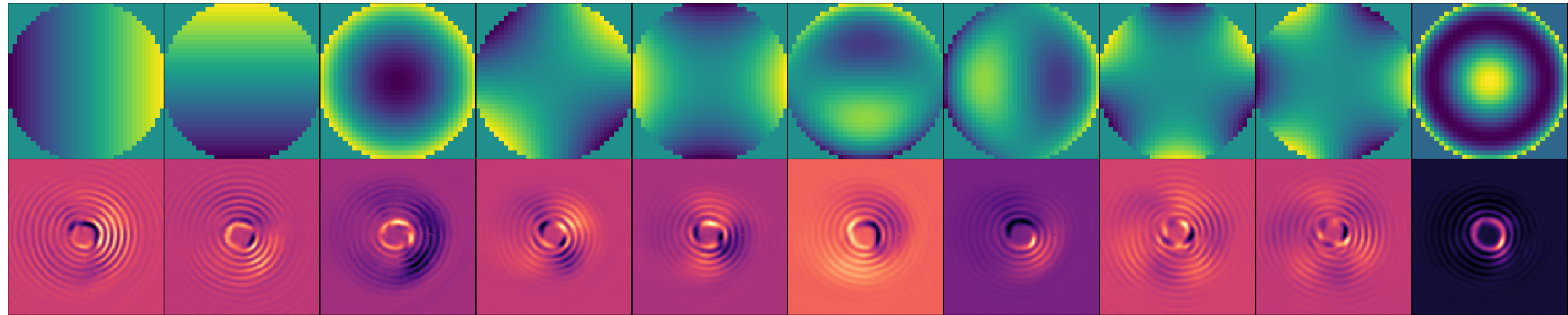
SCoOB Zernike Responses
