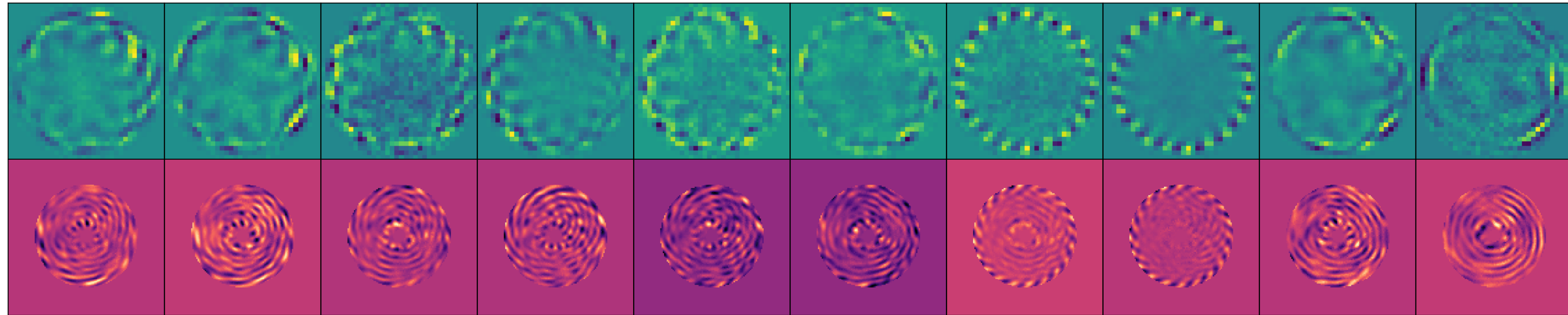
SCoOB HSVD Responses for Modes 100-110
