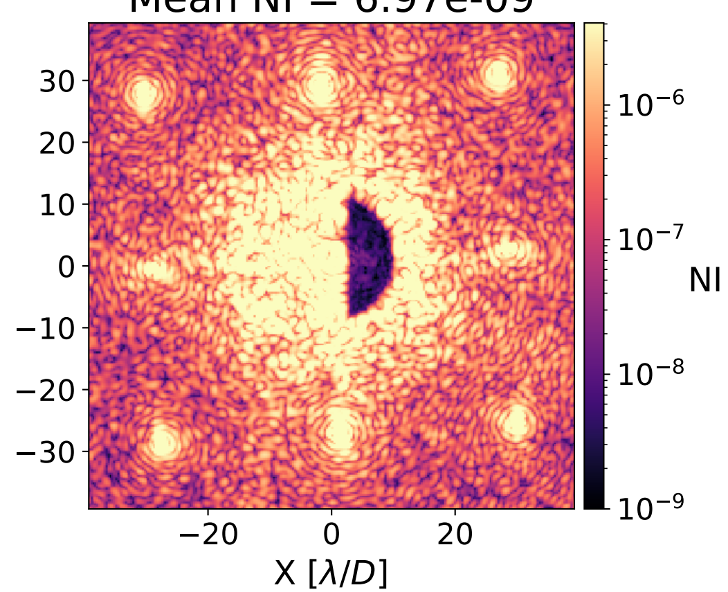
Best Iteration: Mean NI = 6.97\text{e-}09
