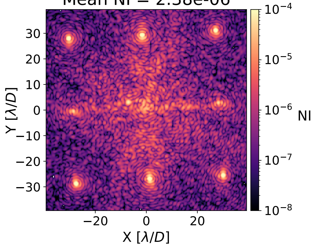
Initial Image: Mean NI = 2.38\text{e-}06
