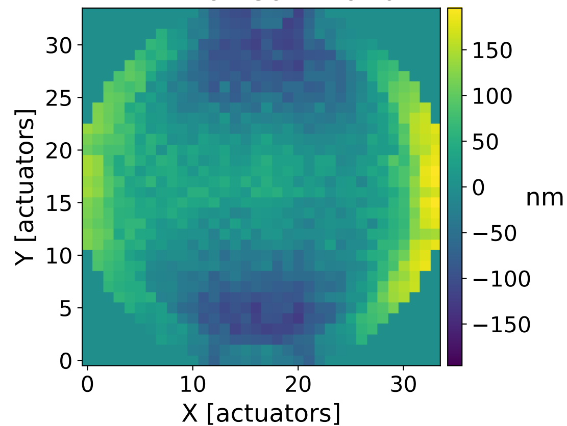
DM Flat Command
