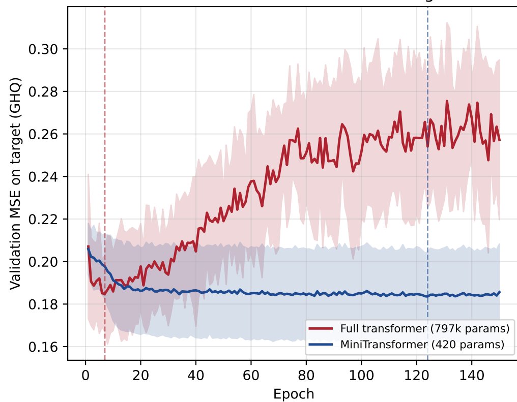
LORA D2: validation MSE on the target
