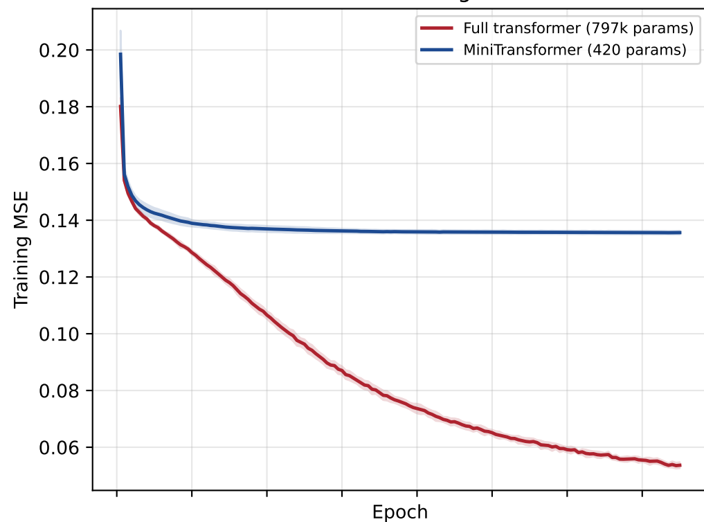
LORA D2: training MSE
