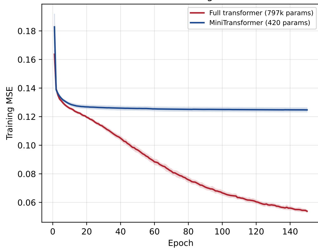
LORA D2: training MSE
