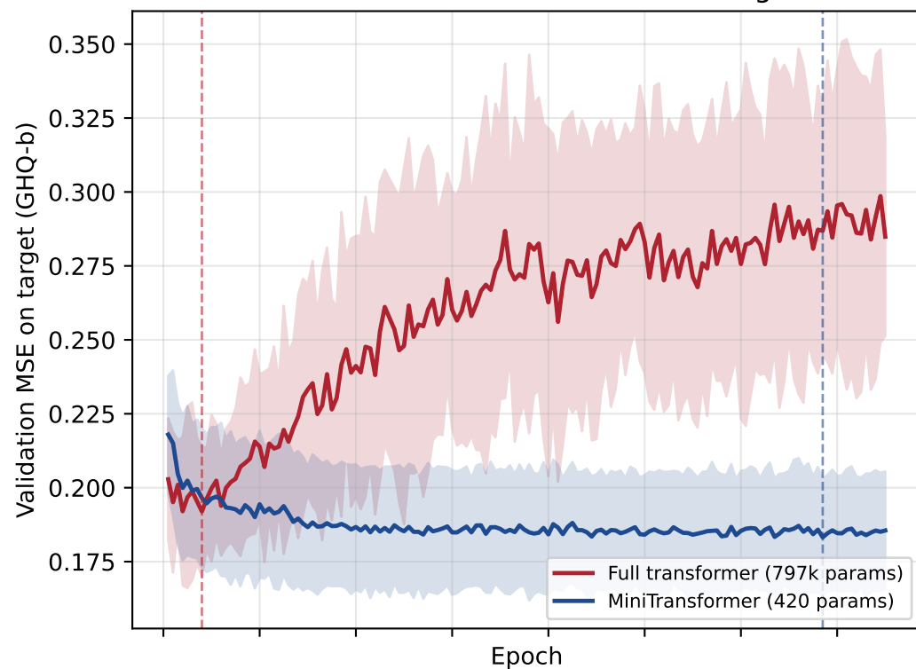
LORA D2: validation MSE on the target
