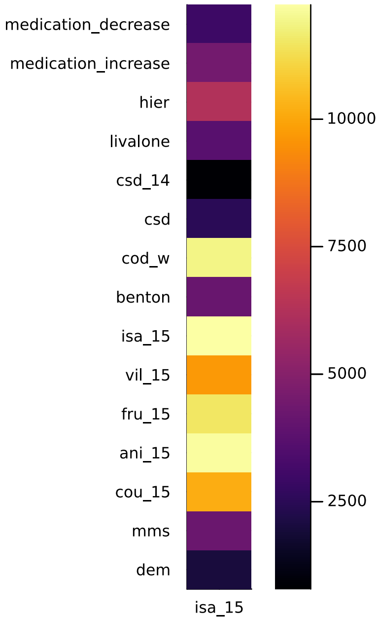
isa_15: lag0
