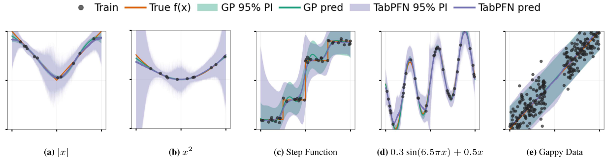
Figure 1 1D Examples: The functions are all adopted from [1]. Each plot has the same x and y axes, both spanning [-0.5, 0.5] . All the GPs are trained on CPU using the defaults of [2] (e.g., constant mean and a Gaussian kernel). TabPFN v2.5 is run on GPU without fine-tuning.
