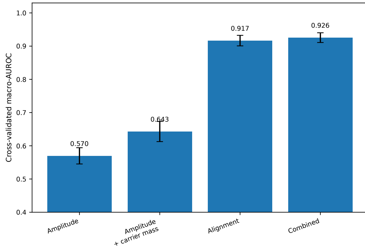
Logistic
