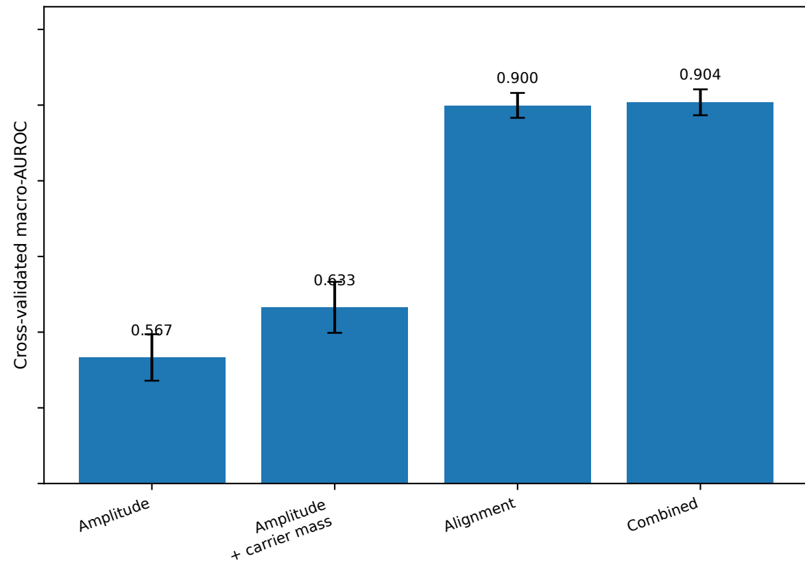
Random forest
