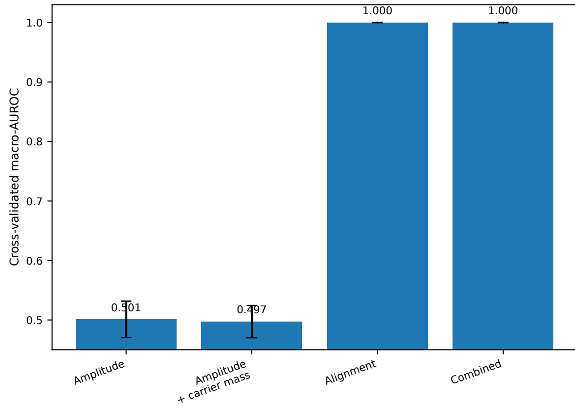
Logistic
