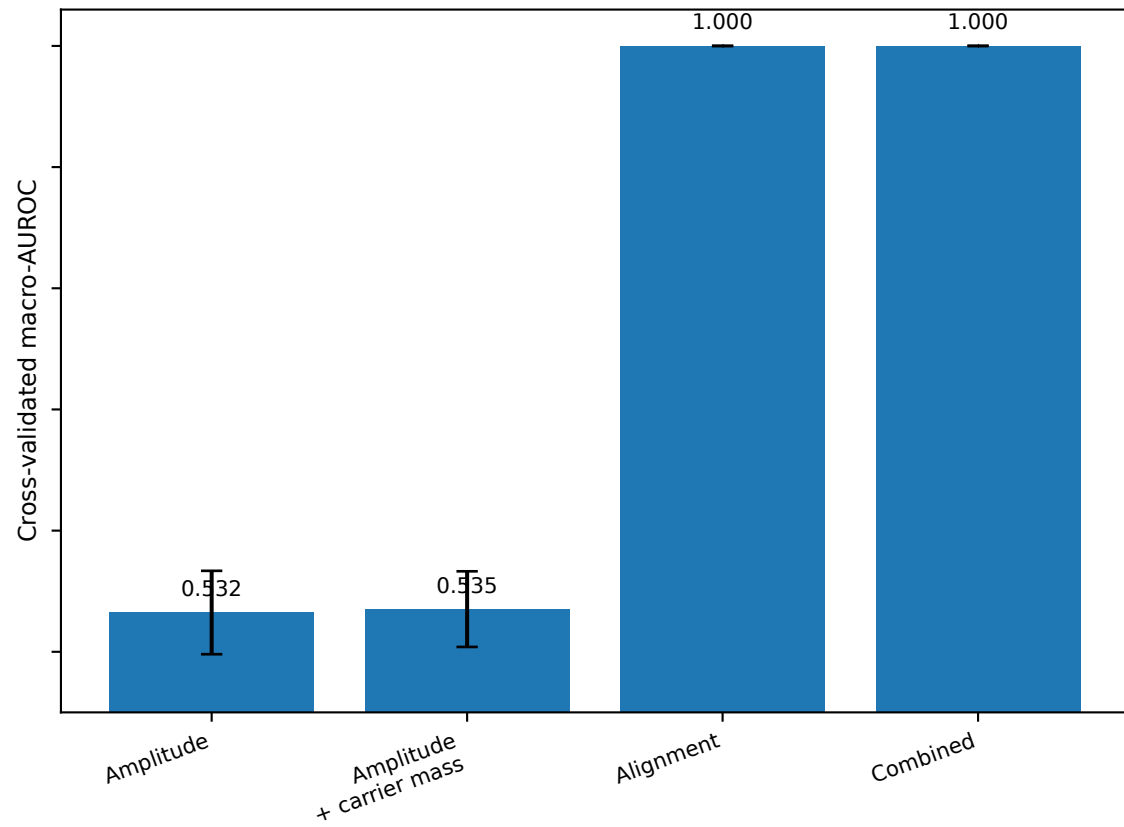
Random Forest
