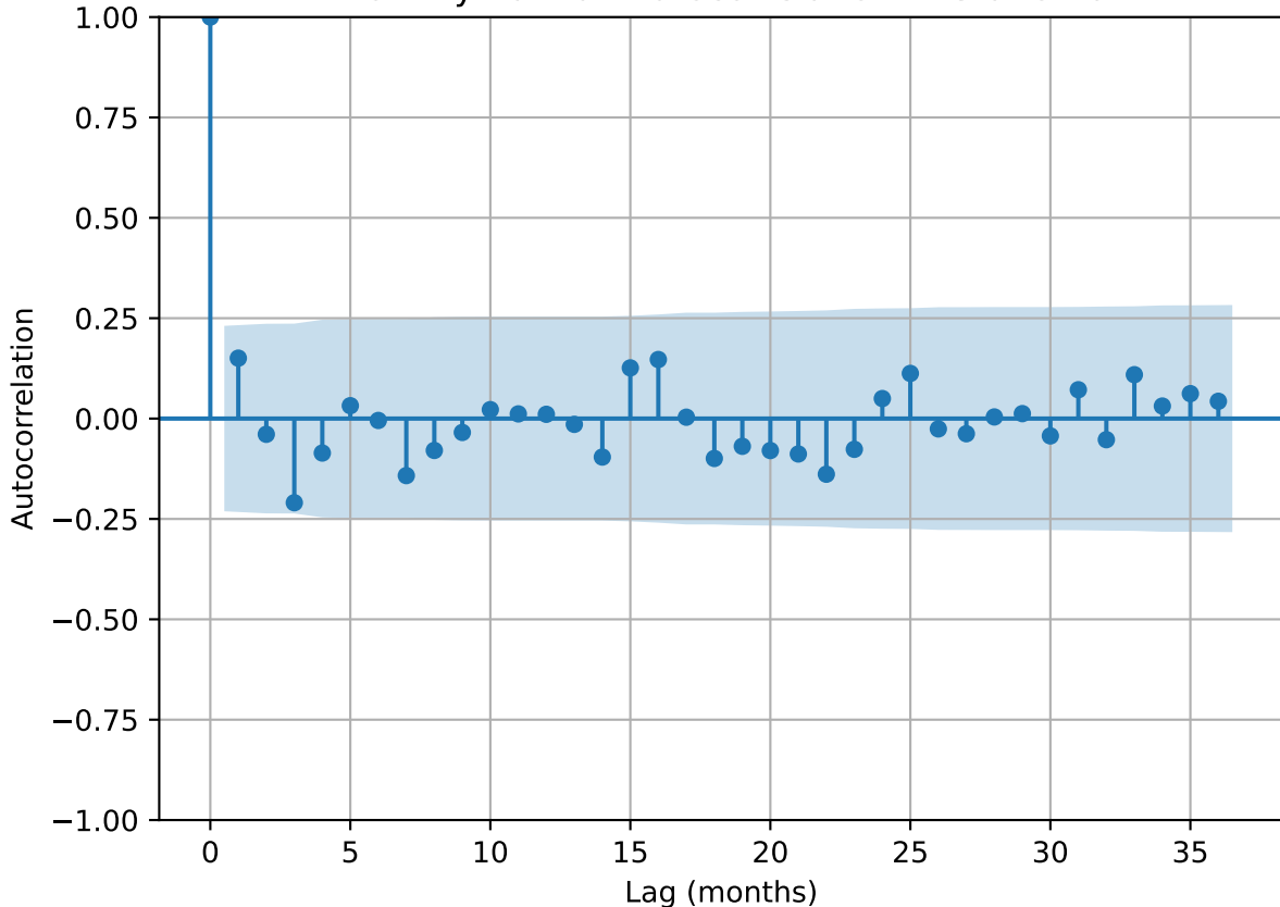
Monthly Rainfall Autocorrelation — Station 6
