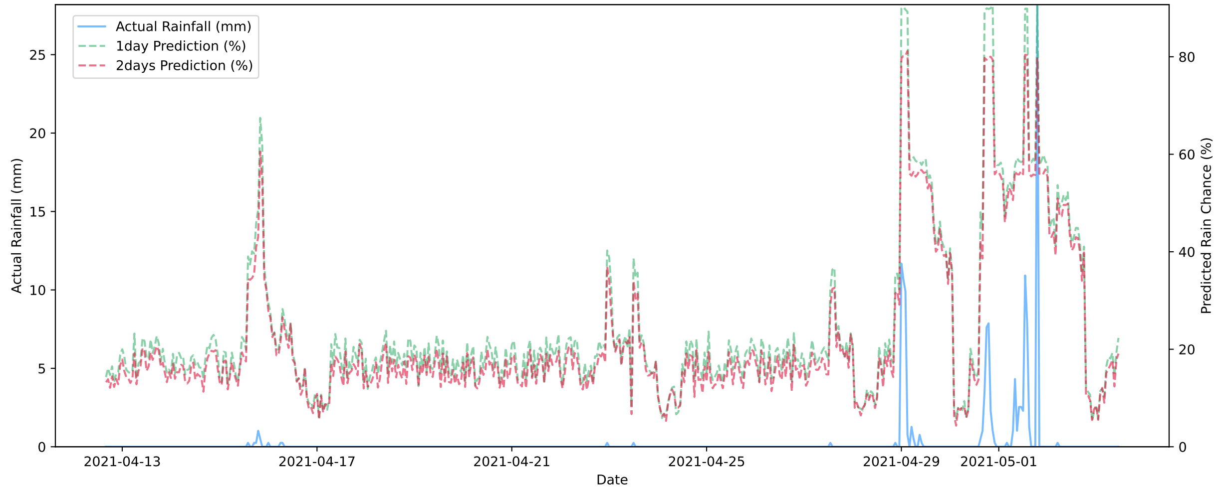
Actual Rainfall vs Predicted Rain Percentage
