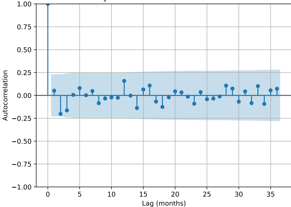
Monthly Rainfall Autocorrelation — Station 2
