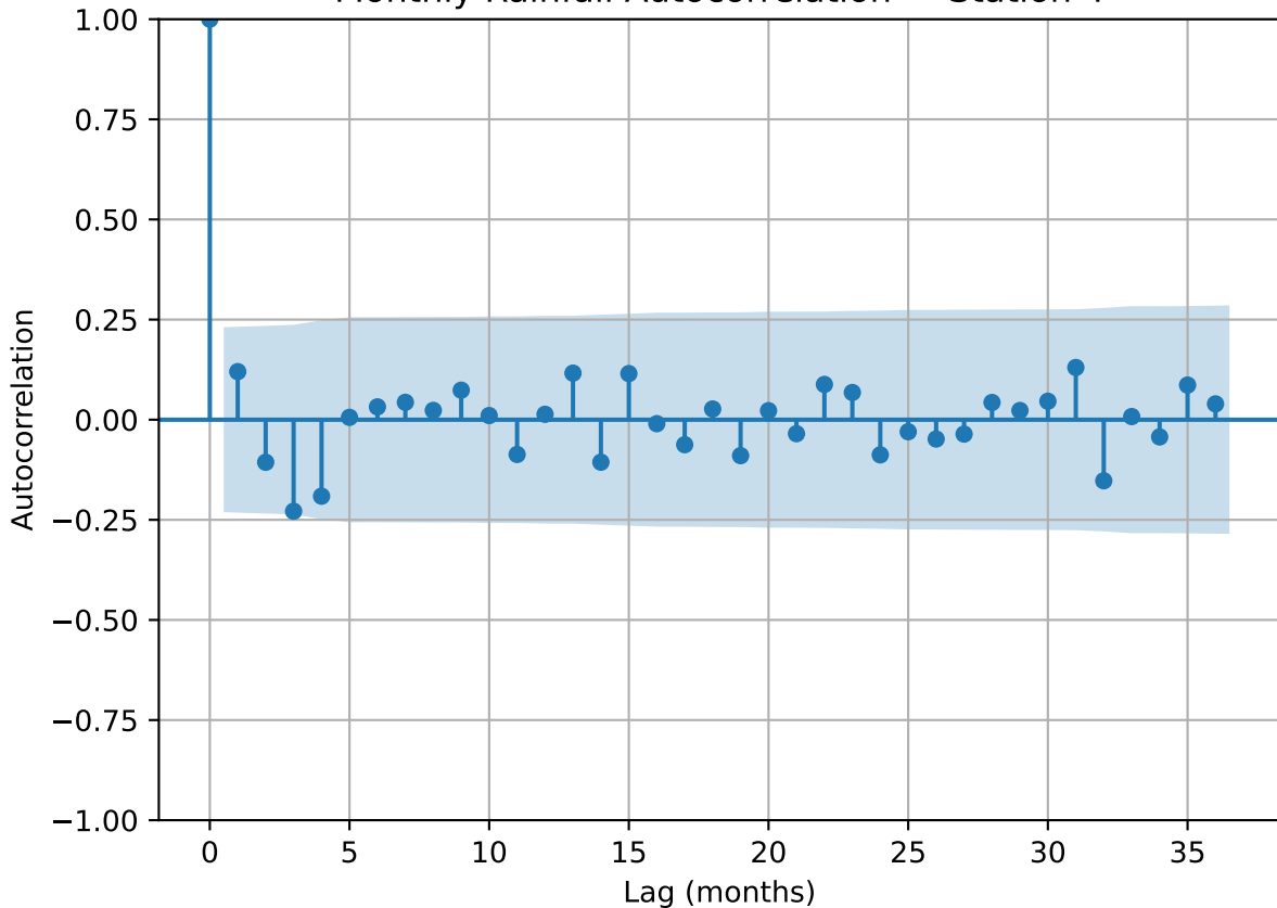
Monthly Rainfall Autocorrelation — Station 4
