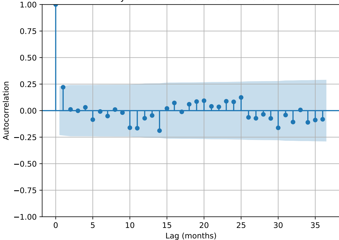
Monthly Rainfall Autocorrelation — Station 1
