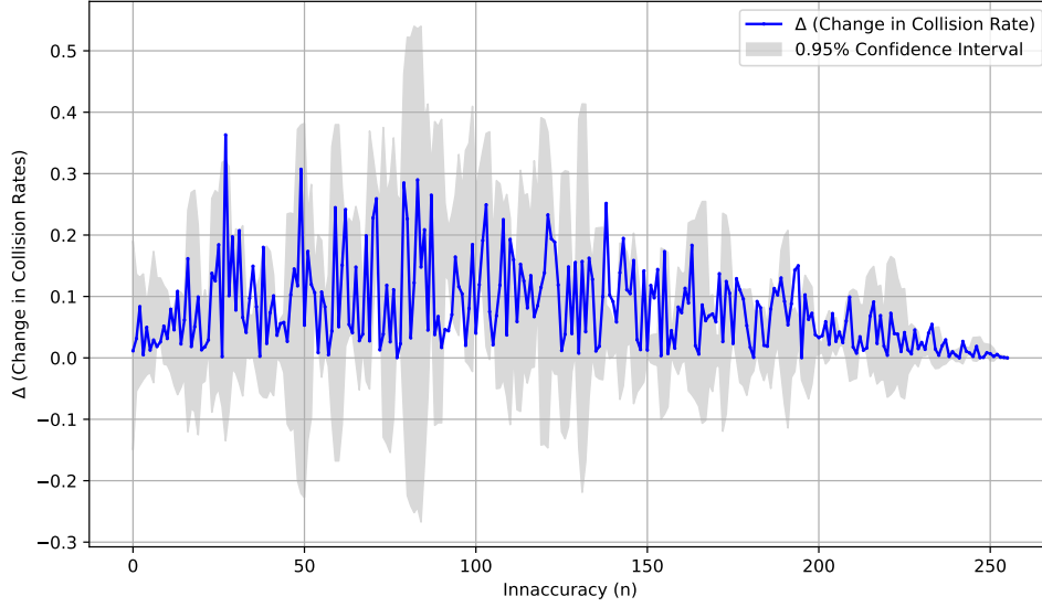
Figure 6: \Delta = |\text{SHA-256} - \text{FullTimePad 2.0}| V.S. Inaccuracy (n)
