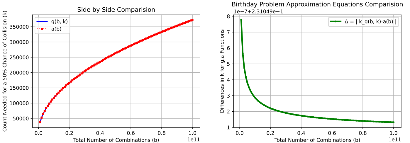
Figure 1: Difference in functions g, a V.S Total Combination
