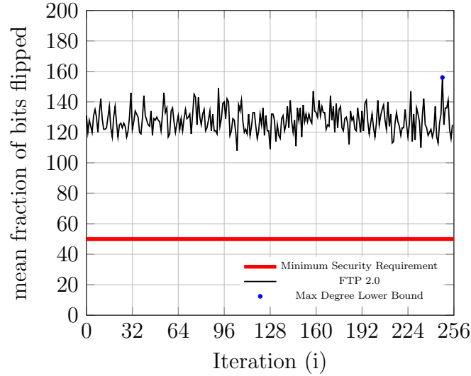
Figure 3: Bit flip probabilities vs. Iteration
