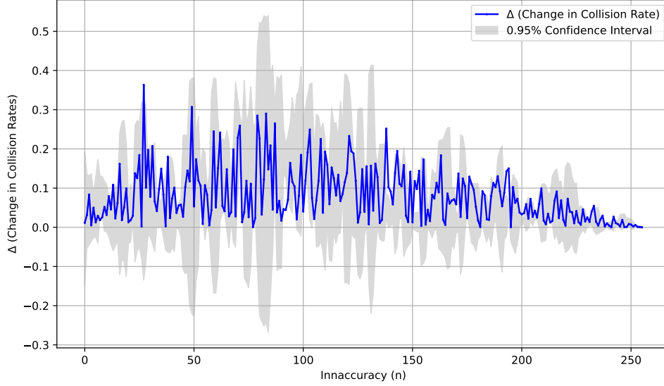
Figure 6: \Delta = |\text{SHA-256} - \text{FullTimePad 2.0}| V.S. Inaccuracy (n)
