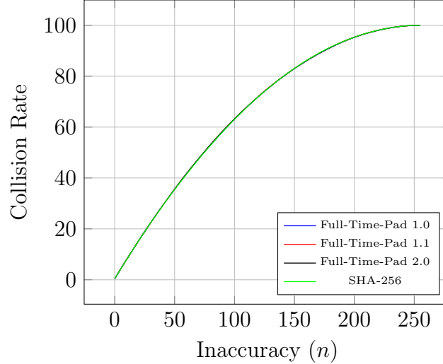
Figure 5: Collision Rate (%) vs. Inaccuracy ( n )
