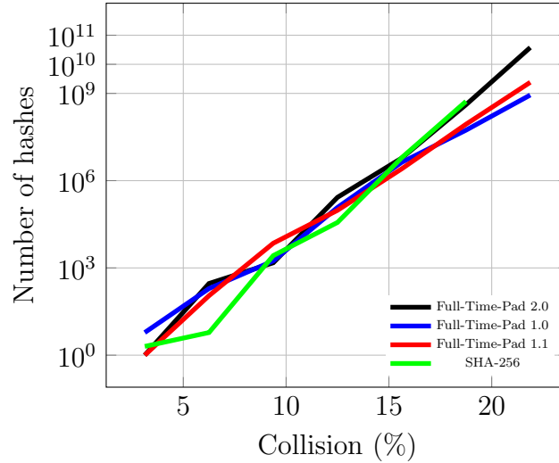
Figure 4: Collision (%) VS. Number of Hashes for Full-Time-Pad
