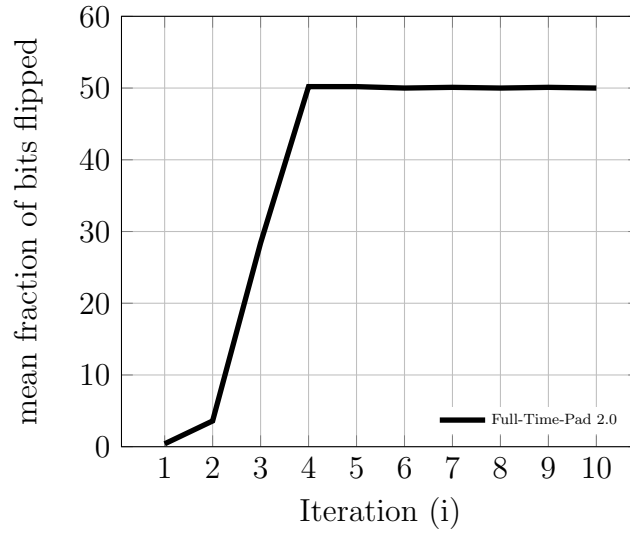
Figure 2: Bit flip probabilities vs. Iteration
