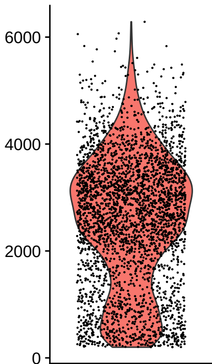
nFeature_RNA
