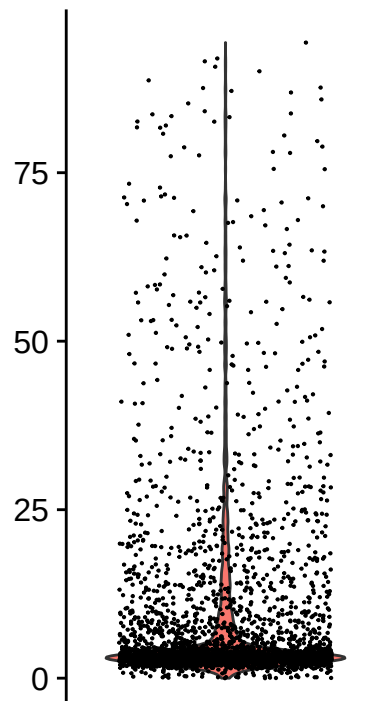
percent.mt
