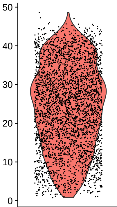
percent.ribo
