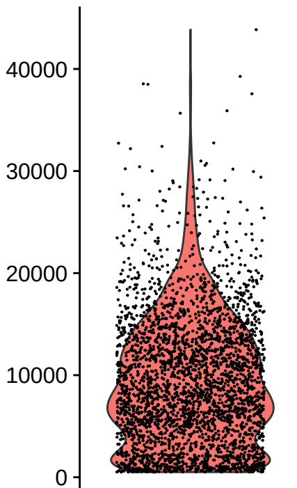
nCount_RNA
