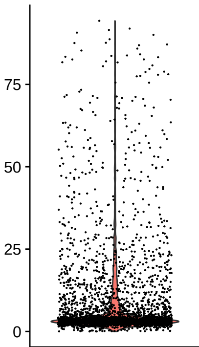
percent.mt
