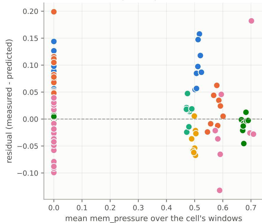
Fit residuals vs system pressure
