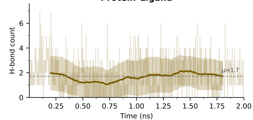
Protein-Ligand
