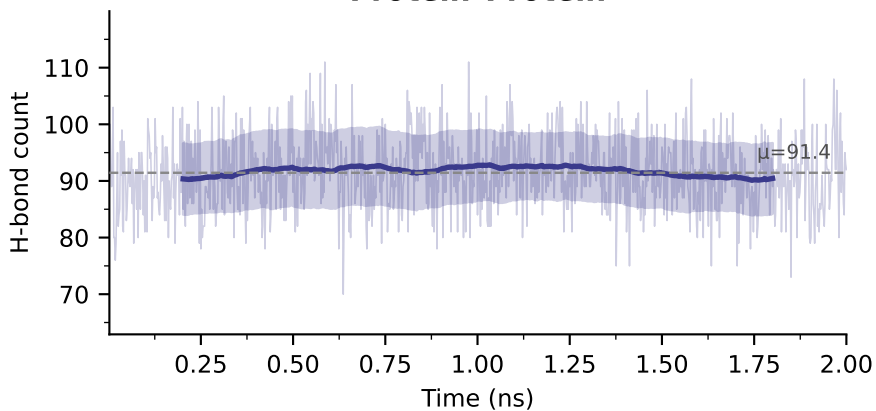
Protein-Protein
