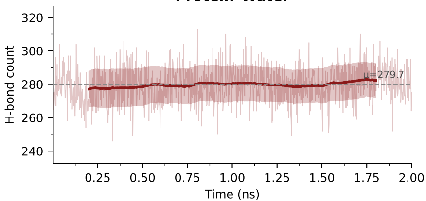
Protein-Water
