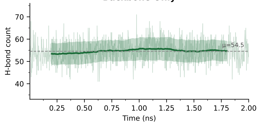
Backbone Only
