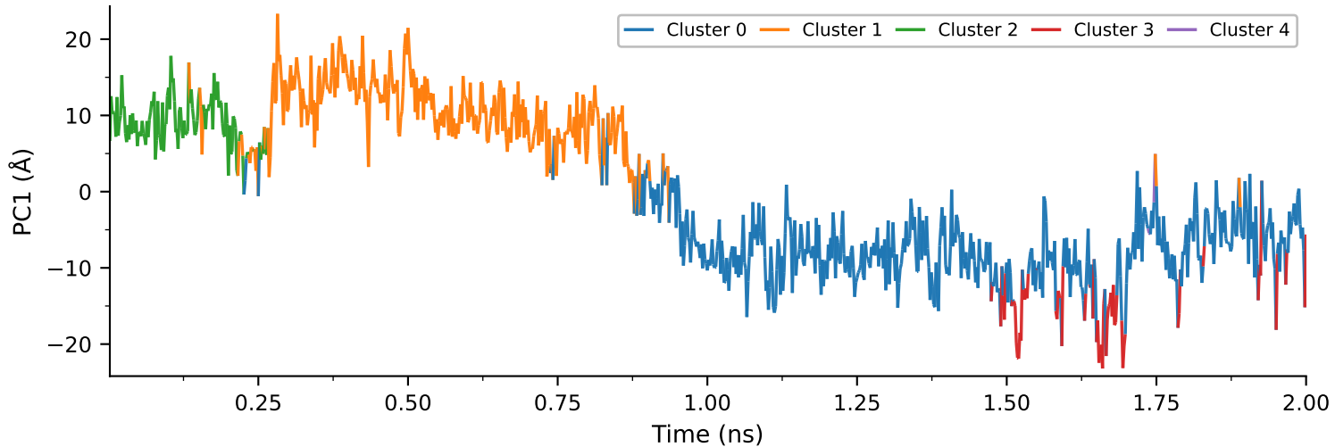
PC1 Time Evolution (colored by cluster)
