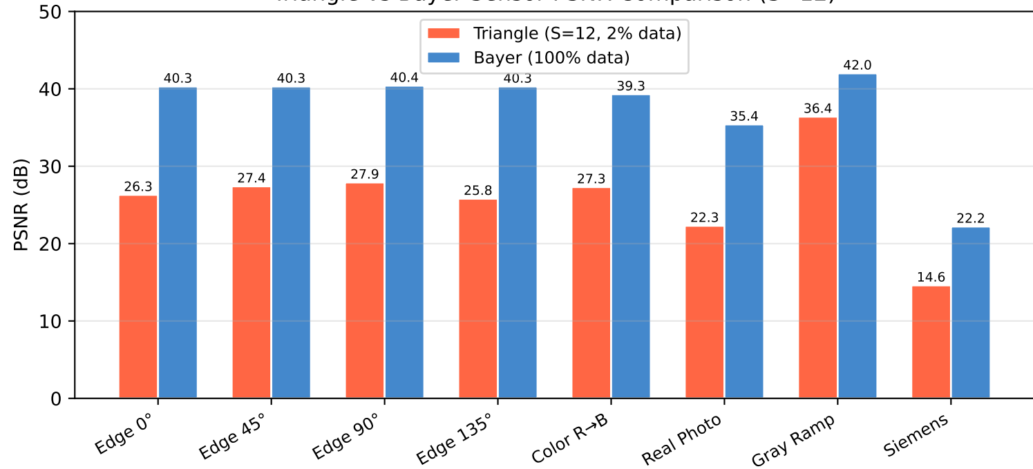
Triangle vs Bayer Sensor PSNR Comparison (S=12)
