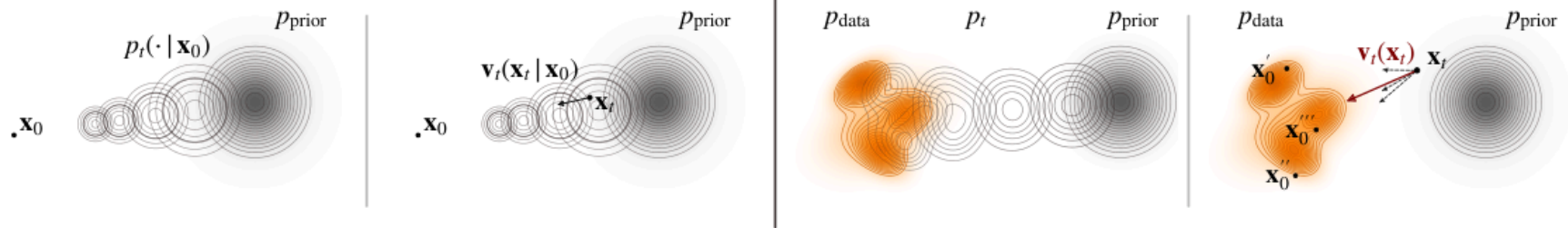
Figure 5.6: Illustration of conditional versus marginal perspectives in diffusion. (This figure is motivated by Lipman et al. (2024).) (1) Conditional Gaussian path p_t(\cdot|\mathbf{x}_0) , showing expanding densities from a fixed \mathbf{x}_0 toward the prior. (2) Conditional velocity \mathbf{v}_t(\mathbf{x}_t|\mathbf{x}_0) = f(t)\mathbf{x}_t - \frac{1}{2}g^2(t)\nabla_{\mathbf{x}_t} \log p_t(\mathbf{x}_t|\mathbf{x}_0) . (3) Marginal density p_t , transporting the data distribution p_{\text{data}} (orange) into the prior p_{\text{prior}} (gray). (4) Marginal velocity \mathbf{v}_t(\mathbf{x}_t) = f(t)\mathbf{x}_t - \frac{1}{2}g^2(t)\nabla_{\mathbf{x}_t} \log p_t(\mathbf{x}_t) .
