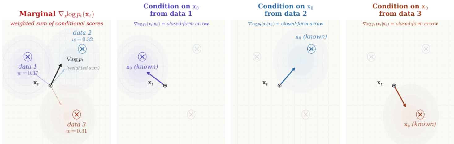
Figure 4.6: Illustration of the denoising score matching trick. The marginal score \nabla_{\mathbf{x}_t} \log p_t(\mathbf{x}_t) is generally an intractable weighted average of the conditional scores over all possible clean samples \mathbf{x}_0 , where the weights are given by the posterior distribution of \mathbf{x}_0 conditioned on the noisy observation \mathbf{x}_t . However, for each fixed \mathbf{x}_0 , the conditional score \nabla_{\mathbf{x}_t} \log p_t(\mathbf{x}_t|\mathbf{x}_0) is available in closed form. Denoising score matching turns this hard marginal estimation problem into an easy per-sample regression problem.
