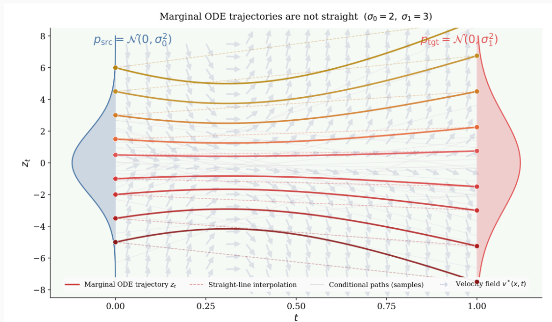
Figure 5.9: Marginal ODE trajectories are not straight under the canonical affine interpolation. We take x_0 \sim \mathcal{N}(0, \sigma_0^2) and x_1 \sim \mathcal{N}(0, \sigma_1^2) with \sigma_0 = 2, \sigma_1 = 3 , and independent coupling. Gray lines show sampled conditional paths (1-t)x_0 + tx_1 , which are straight by construction. Solid curves show the exact marginal ODE trajectories z_t = z_0 \sqrt{(1-t)^2 + (\sigma_1/\sigma_0)^2 t^2} , and dashed lines show the corresponding straight-line interpolations from z_0 to z_1 . The visible gap between
