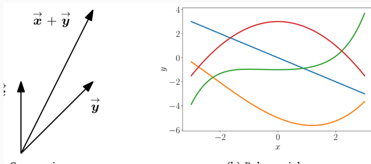
Figure 2.1 Different types of vectors. Vectors can be surprising objects, including (a) geometric vectors and (b) polynomials.
