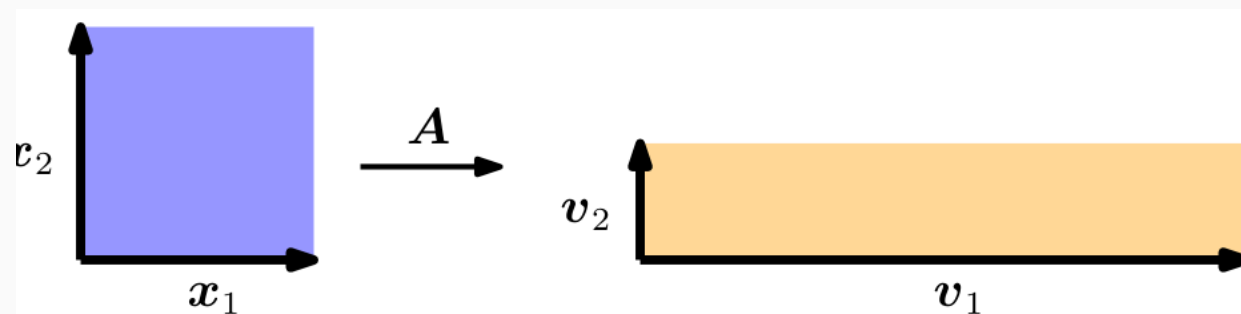
Figure 4.6 Geometric interpretation of eigenvalues. The eigenvectors of A get stretched by the corresponding eigenvalues. The area of the unit square changes by |\lambda_1 \lambda_2| , the perimeter changes by a factor of \frac{1}{2}(|\lambda_1| + |\lambda_2|) .
