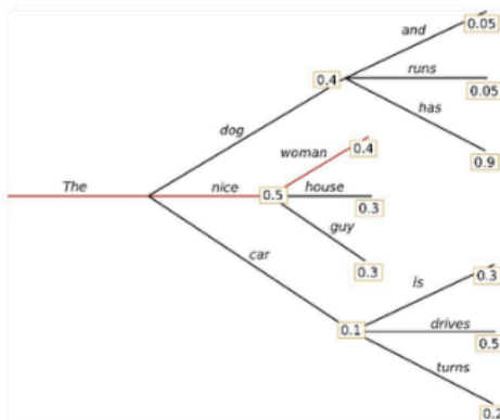
Greedy
