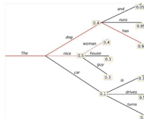
Beam
