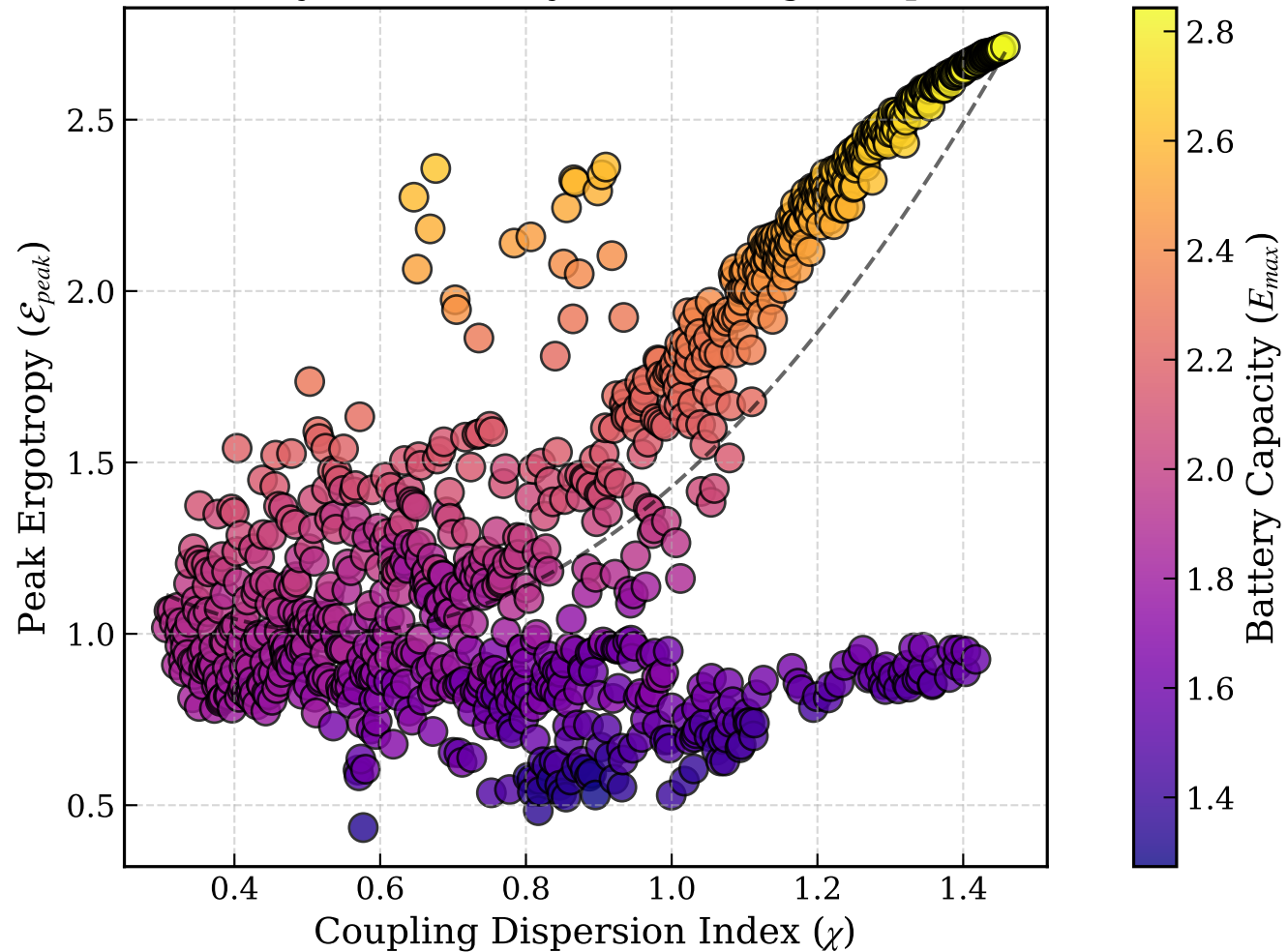
Thermodynamic Purity Loss at High Dispersion
