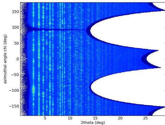
Figure 2. 2D-regrouped image without pixel splitting. Note the missing pixels near the beam stop and the high-frequency noise patterns.
