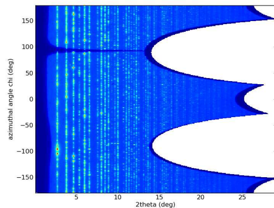
Figure 3. 2D-regrouped image with pixel splitting. The transformation of a smooth image remains smooth.
