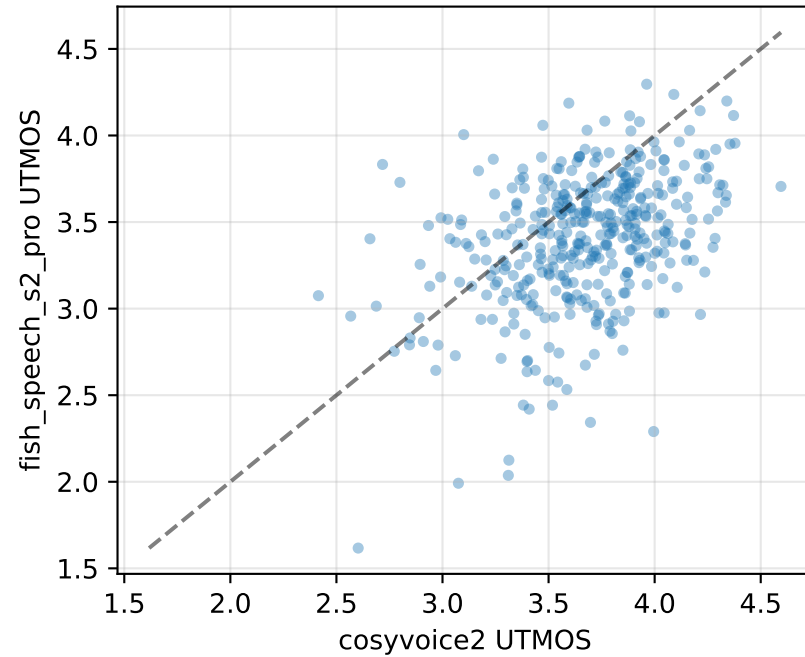
cosyvoice2 vs fish_speech_s2_pro
