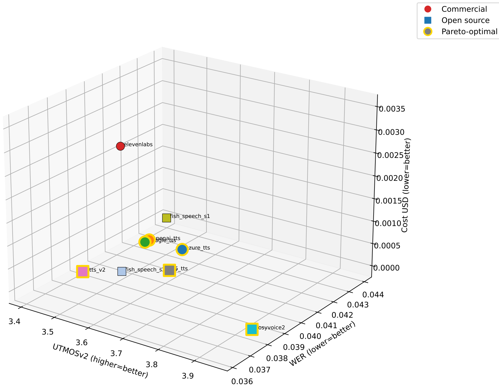
3D Pareto projection — tts
