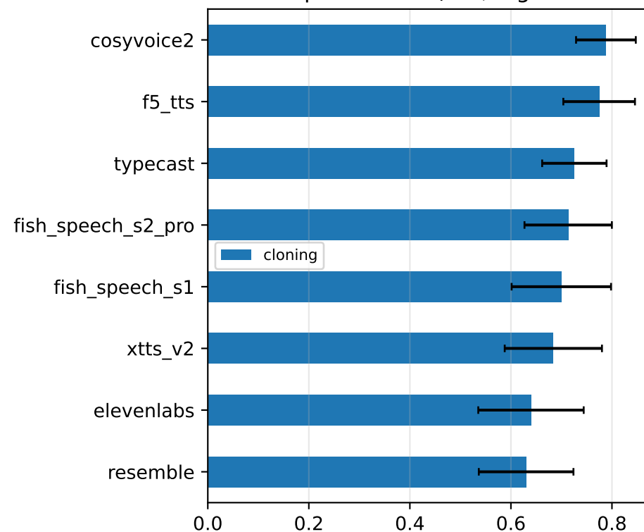
ECAPA speaker sim (0-1, higher better)
