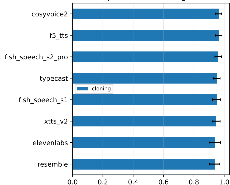
WavLM speaker sim (0-1, higher better)
