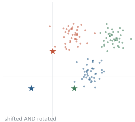
(b) new user, raw features
