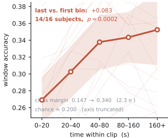
(b) SEED-V ( n = 16 )
