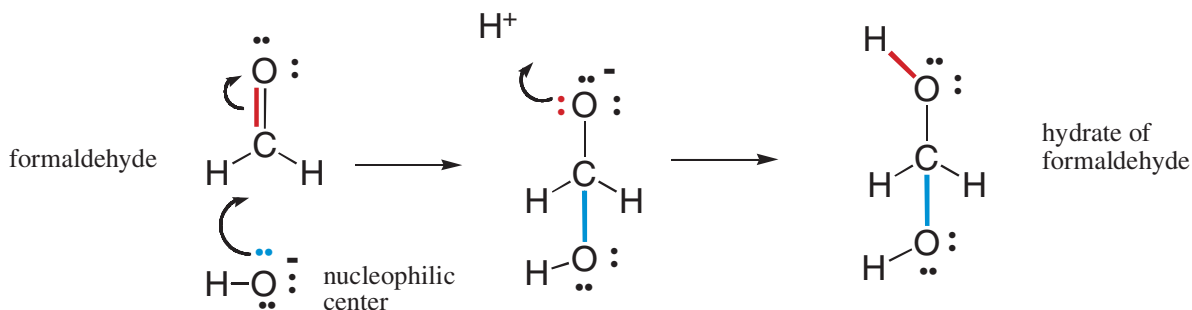
FIGURE 2.5 Reaction of the electrophilic carbon of formaldehyde with the nucleophilic oxygen of hydroxide gives the hydrate of formaldehyde. Note the concerted formation of a new bond (blue) using the unshared pair of electrons (also blue) on the oxygen nucleophilic center with the breaking of a bond (red). This bond breaking delivers an unshared pair of electrons (red) to the oxygen intermediate. These electrons can form a new bond (red) to an electrophilic proton.
