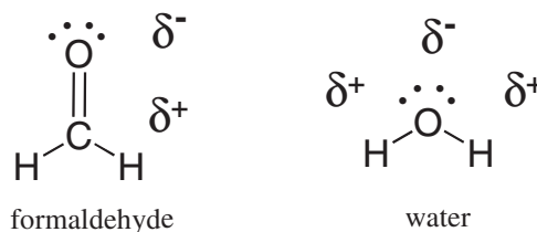
FIGURE 2.3 The oxygen atom is more electro-negative than either carbon or hydrogen. Therefore, the bonds between oxygen and these atoms are polarized to place a fractional negative charge (indicated by \delta^- ) on the oxygen atom and a fractional positive charge (indicated by \delta^+ ) on the carbon or hydrogen atoms.
