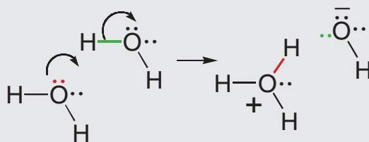
FIGURE 2.2.1 Two curved arrows can be written to show the transfer of a proton from one water molecule to another to give the hydronium ion ( \text{H}_3\text{O}^+ ) and the hydroxide ion ( \text{HO}^- ). The oxygen carrying the red electrons is the nucleophilic center. It brings the electron pair that is to form the new bond (red). The hydrogen attached to the oxygen in the second water molecule via the green bond is the electrophilic center.
