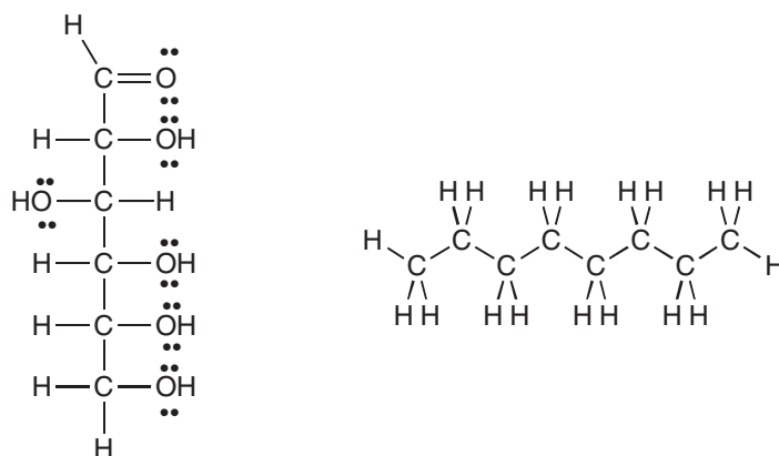
FIGURE 2.4 Structures of glucose (left) and octane (right). Given the large number of dipolar C-O bonds and the large number of nonbonding electrons (the dots in the structure), one expects glucose to be a hydrophilic molecule that dissolves well in water. In contrast, octane can be seen, by its structure, to contain only nondipolar C-C and C-H bonds, and no unshared electron pairs. Therefore, octane is expected to be a hydrophobic compound insoluble in water.
