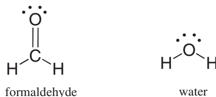
FIGURE 2.1 Lewis structures for formaldehyde (left) and water (right) show the presence of four electrons (each represented by a dot) on the oxygen atoms of the two molecules. These electrons are not involved in the formation of any bond. The pairs of electrons involved in holding the molecule together are represented by lines.
