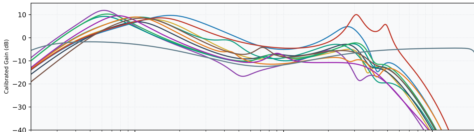
'65 Fender Bassman (AA864) (T=5, M=5, B=5) — Blackface Bassman; 100nF deep bass cap, 47nF mid cap, 100k slope [Norm: +6.5 dB]
