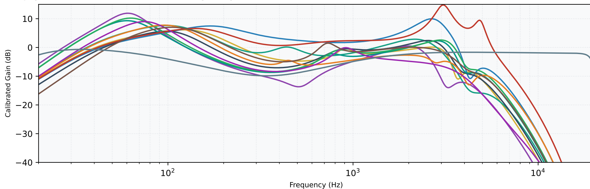
Cabinet Models (12 Discrete Enclosures)
