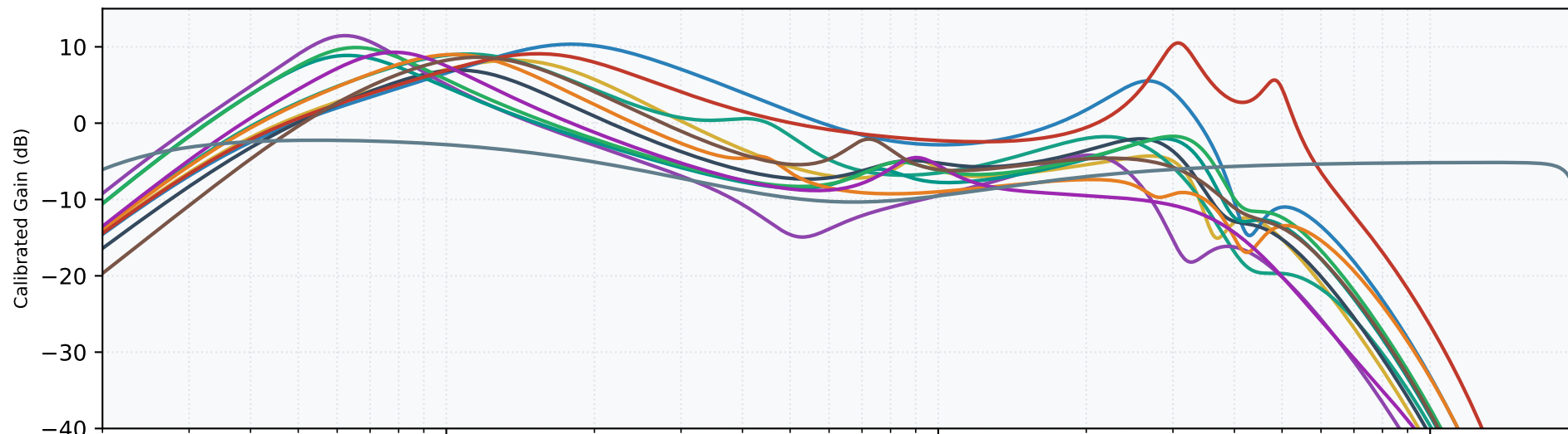
Vox AC30 Top Boost (T=5, M=5, B=5) — British chime; 47pF small treble cap, 100k slope, sparkling highs [Norm: +0.2 dB]
