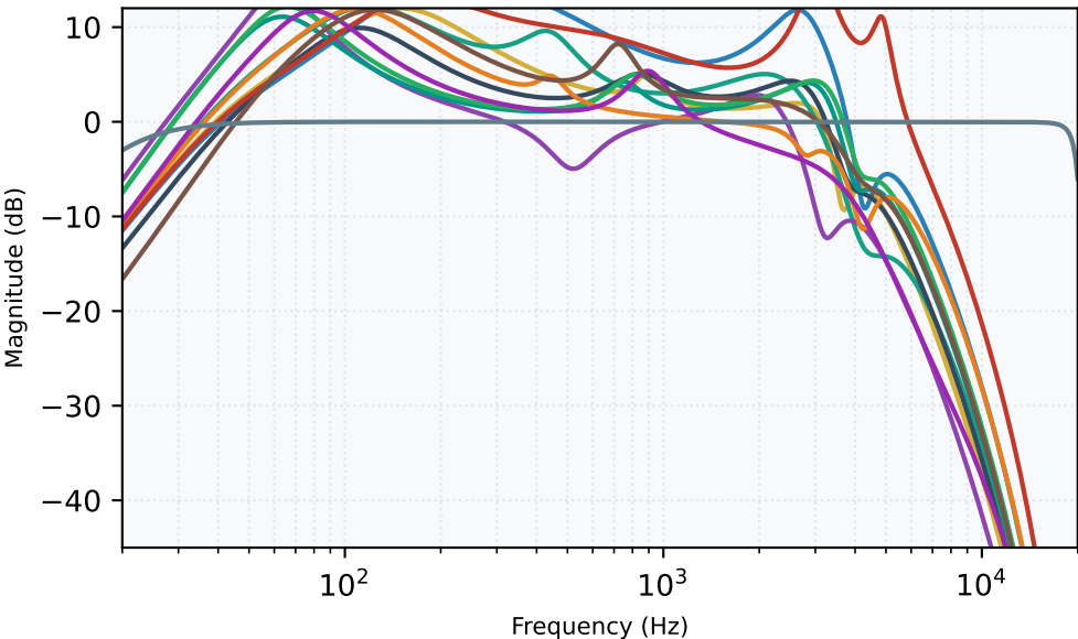
Cabinet Enclosure Frequency Response
