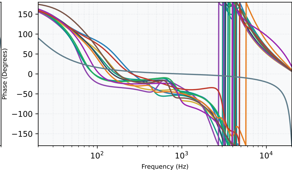
Cabinet Phase Responses
