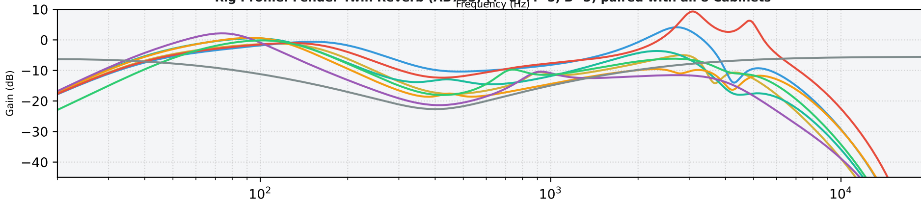
Rig Profile: Fender Twin Reverb (AB763) (T=5, M=5, B=5) paired with all 8 Cabinets
