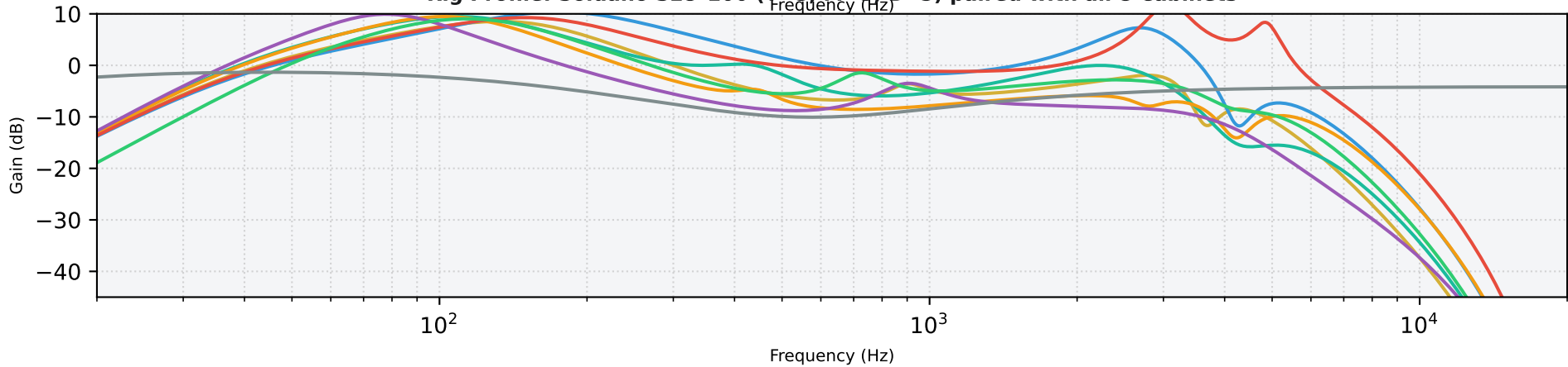
Rig Profile: Soldano SLO-100 (T=5, M=5, B=5) paired with all 8 Cabinets
