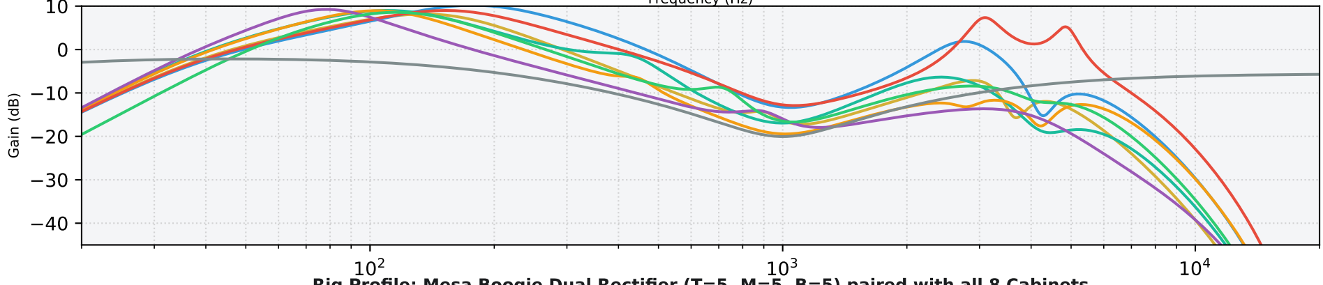
Rig Profile: Mesa Boogie Dual Rectifier (T=5, M=5, B=5) paired with all 8 Cabinets
