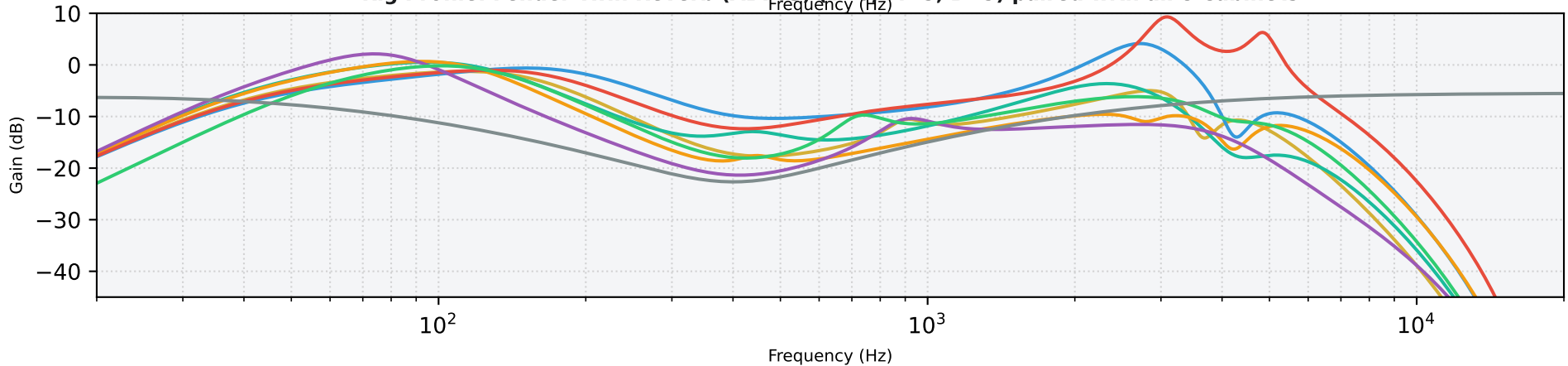
Rig Profile: Fender Twin Reverb (AB763) (T=5, M=5, B=5) paired with all 8 Cabinets
