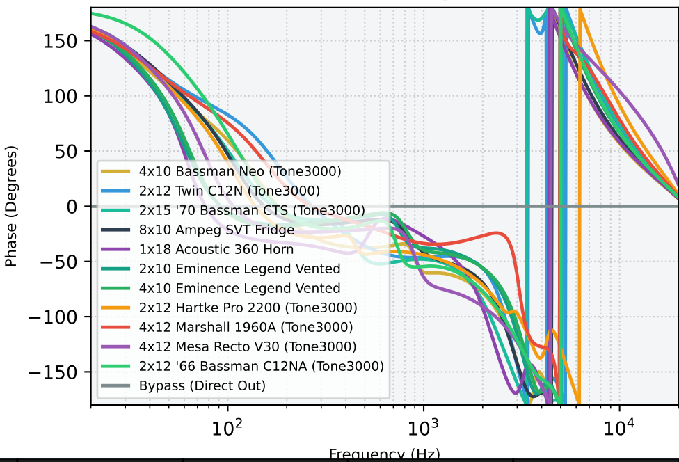
Cabinet Phase Responses
