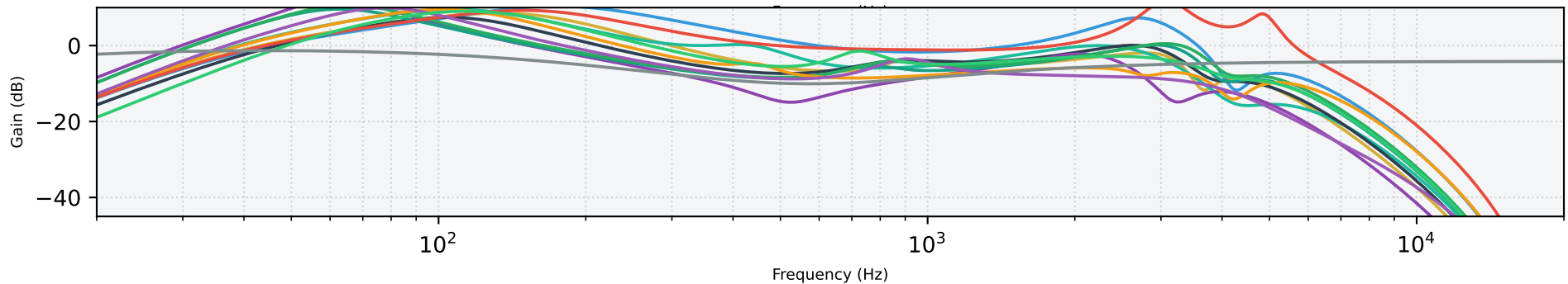
Rig Profile: Soldano SLO-100 (T=5, M=5, B=5) paired with all 12 Cabinets
