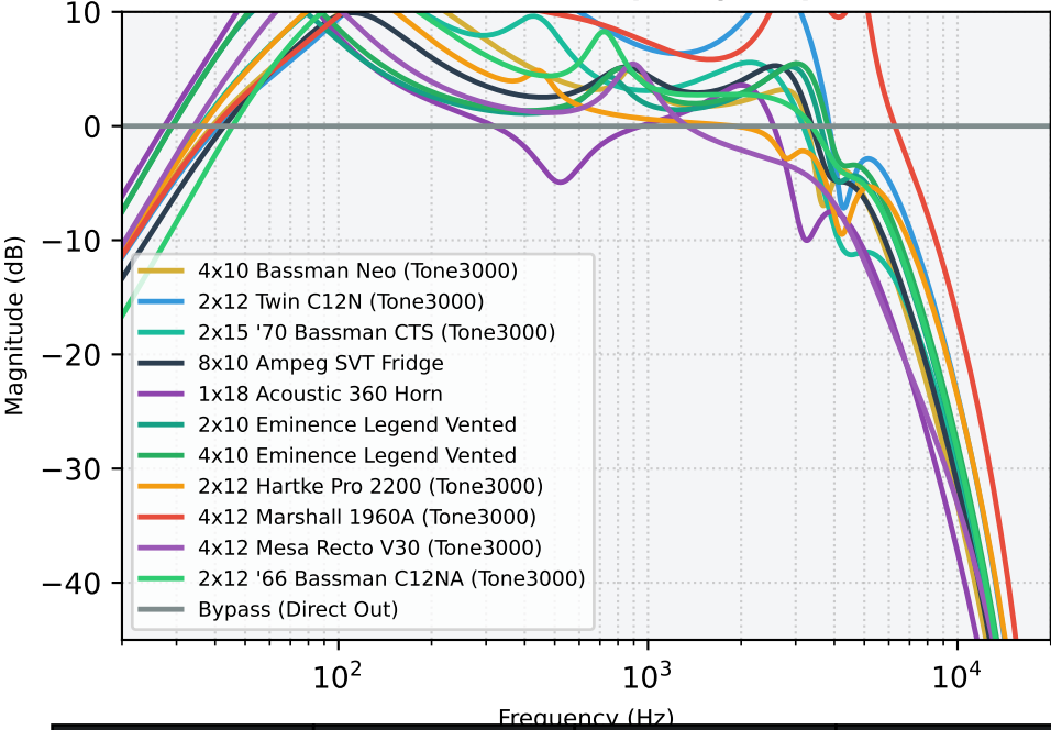
Cabinet Enclosure Frequency Response
