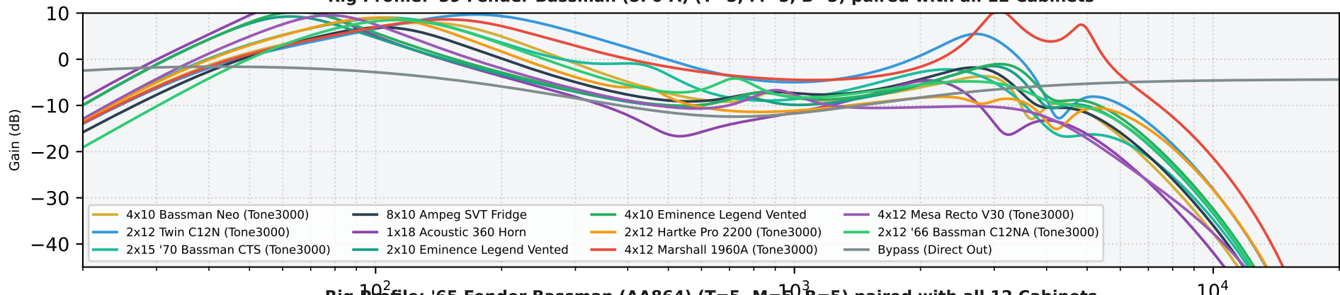
Rig Profile: '65 Fender Bassman (AA864) (T=5, M=5, B=5) paired with all 12 Cabinets
