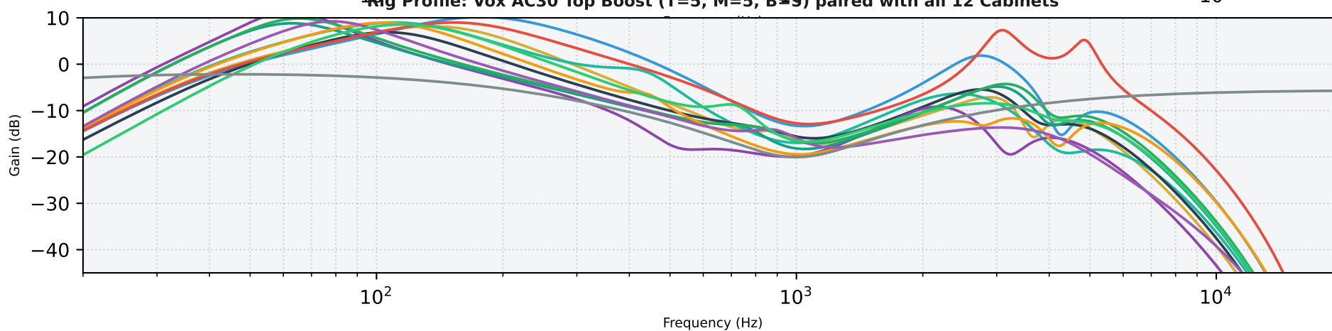
Rig Profile: Vox AC30 Top Boost (T=5, M=5, B=5) paired with all 12 Cabinets
