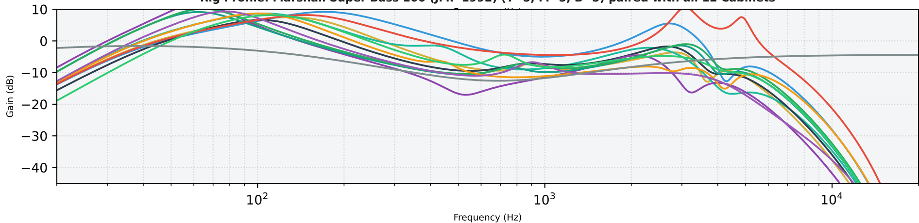
Rig Profile: Marshall Super Bass 100 (JMP 1992) (T=5, M=5, B=5) paired with all 12 Cabinets
