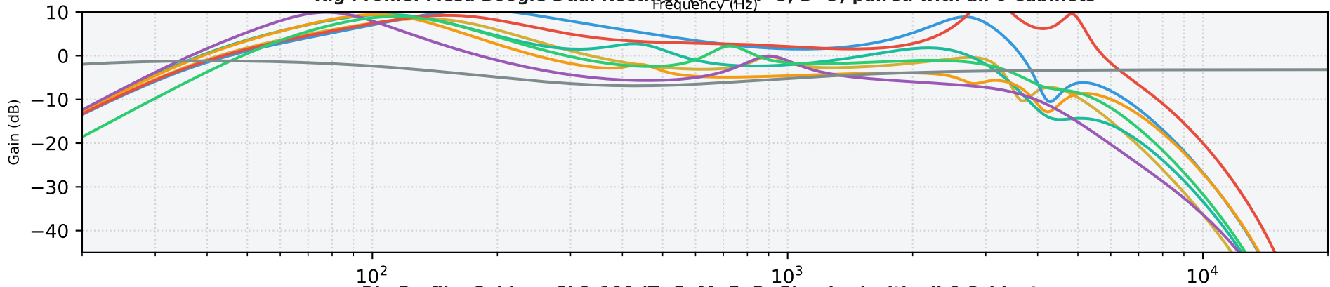
Rig Profile: Soldano SLO-100 (T=5, M=5, B=5) paired with all 6 Cabinets
