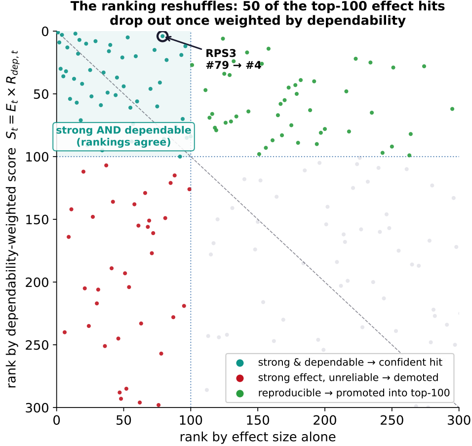
Figure 1: Rank by effect size alone (horizontal) against rank by the dependability-weighted score (vertical); the dotted lines mark the top 100 on each axis. The upper-left quadrant holds targets that are both strong and dependable, where the two rankings agree; lower-left targets are strong but unreliable and are demoted; upper-right targets are reproducible and are promoted. RPS3 is circled.
