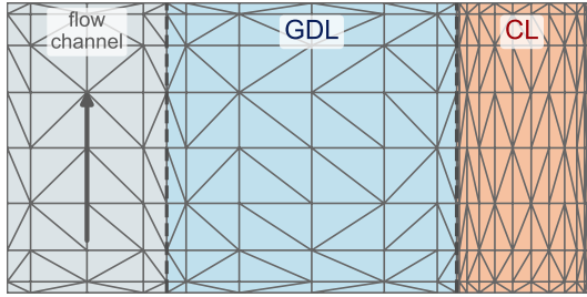
(b) Model layout: flow channel + GDL/CL
