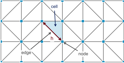
(a) Triangular mesh (2D)
